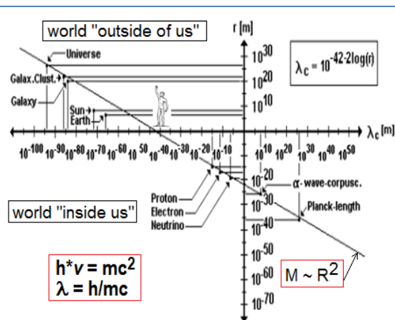
Fig. 2: Stable objects relations in the global space.
