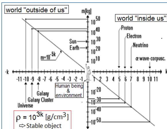
Fig. 1: Mass of stable objects in function of number k \Rightarrow integer value
